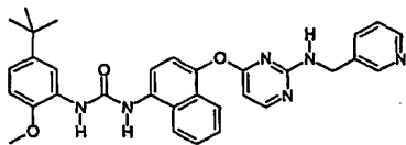
1-(5-tert-Butyl-2-methoxy-phenyl)-3-(4-{2-[(pyridin-3-ylmethyl)amino]-pyrimidin-4-yloxy}-naphthalen-1-yl)-urea;
